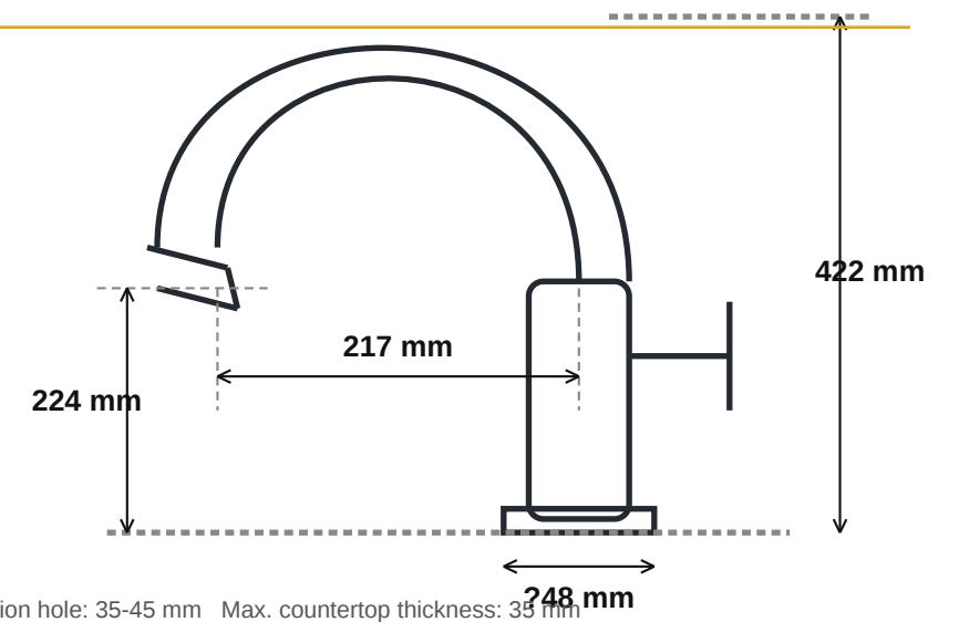
DIAGRAM (Unit: mm)
