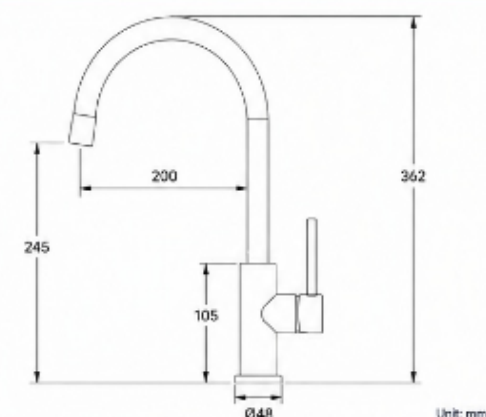
DIAGRAM (Unit: mm)
